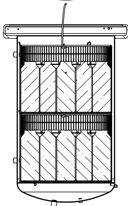
SECTION G-G
