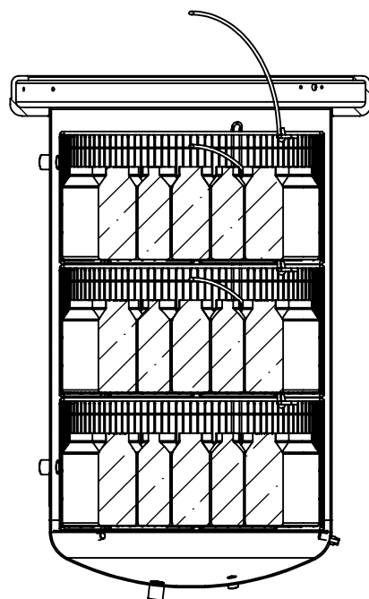
SECTION C-C
